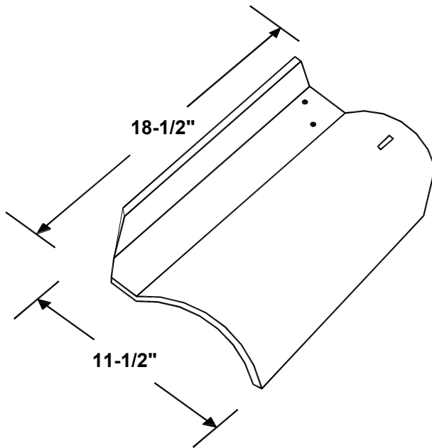
AMAZONA SPANISH "S" CLAY ROOF TILE
