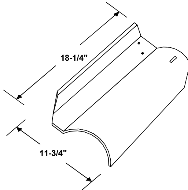
ARIZONA SPANISH "S" CLAY ROOF TILE
