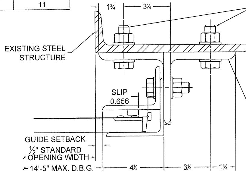
9 GUIDE ASSEMBLY STEEL STRUCTURE (Z-GUIDE OR E-GUIDE)
