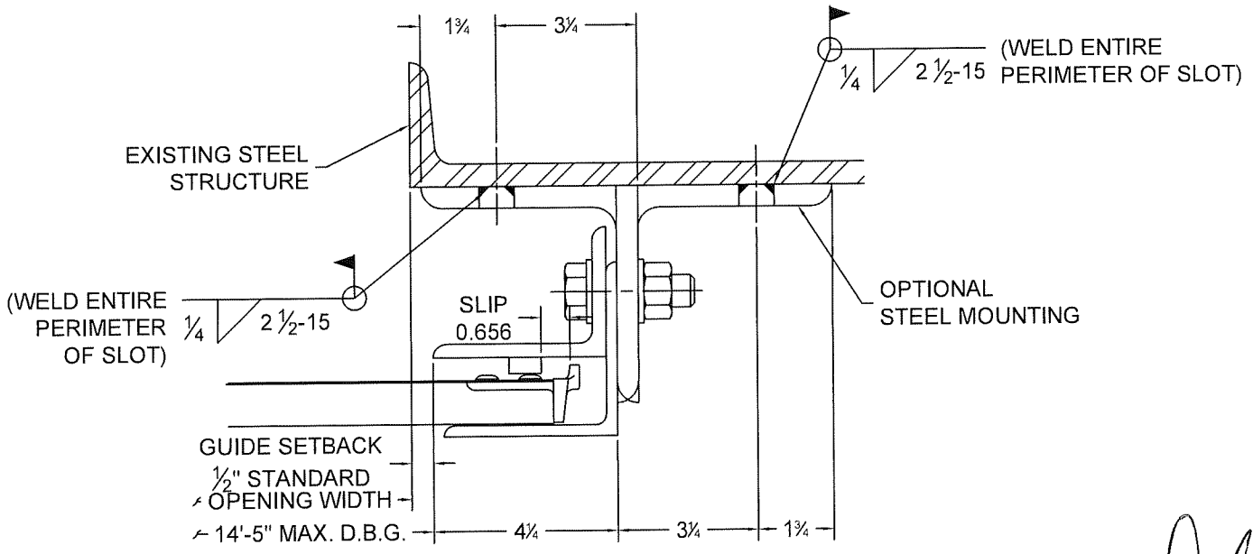
10 GUIDE ASSEMBLY STEEL STRUCTURE (Z-GUIDE OR E-GUIDE)
