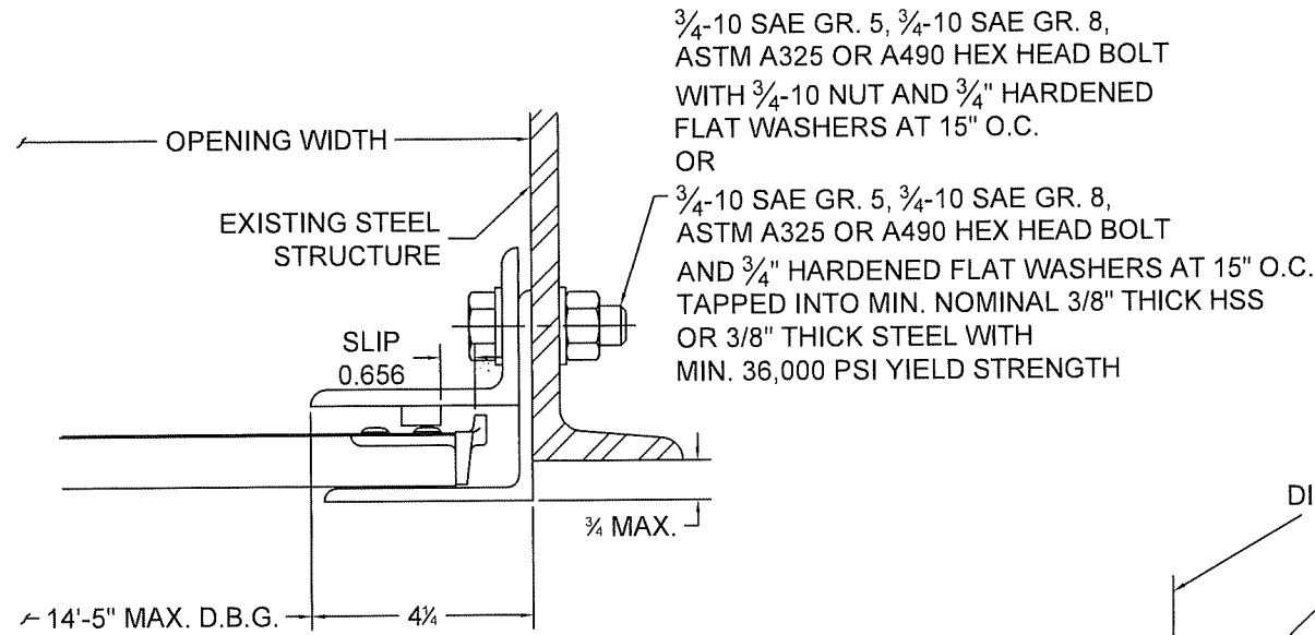
12 GUIDE ASSEMBLY STEEL STRUCTURE (BETWEEN JAMBS GUIDE)
