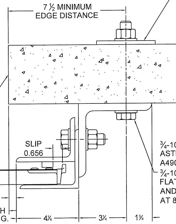
11 GUIDE ASSEMBLY FILLED BLOCK STRUCTURE (Z-GUIDE)
