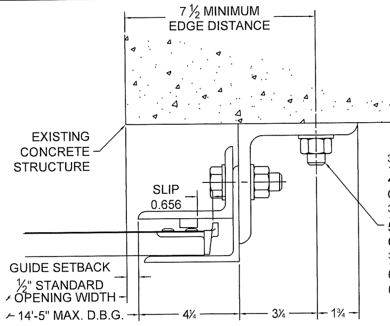
8 GUIDE ASSEMBLY CONCRETE STRUCTURE (Z-GUIDE)
