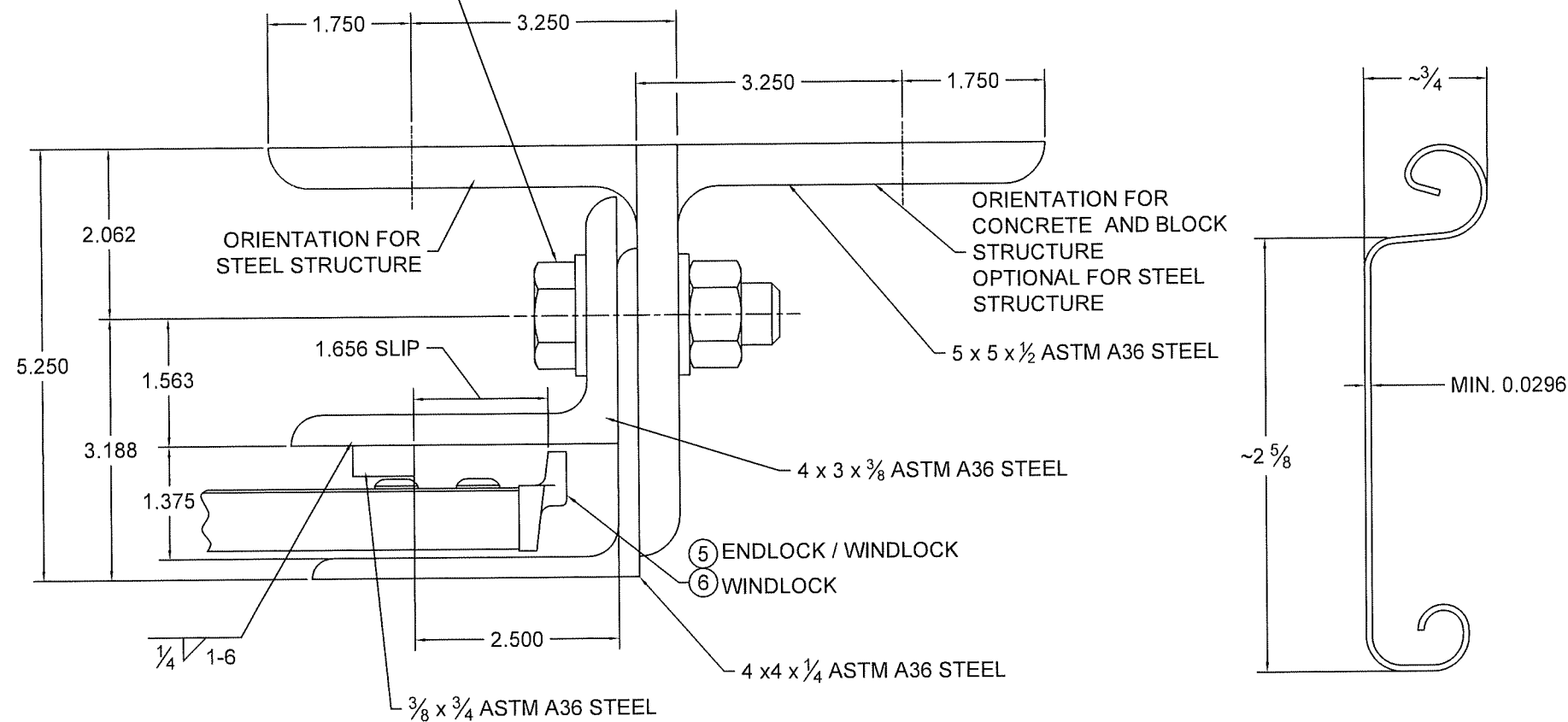
③ SLAT DETAIL TYPICAL SECTION
