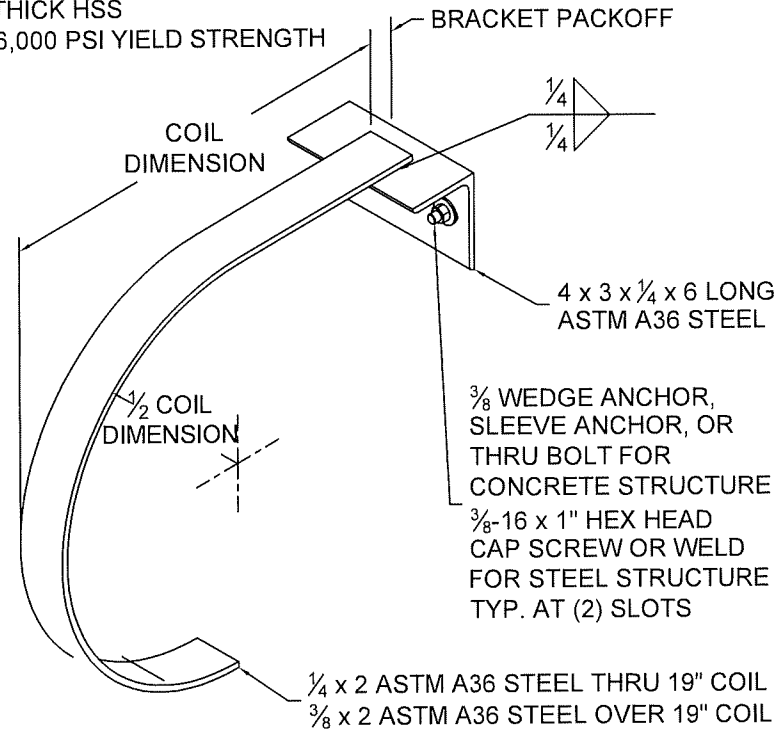
14 MID-HOOD SUPPORT (WHEN REQUIRED)
