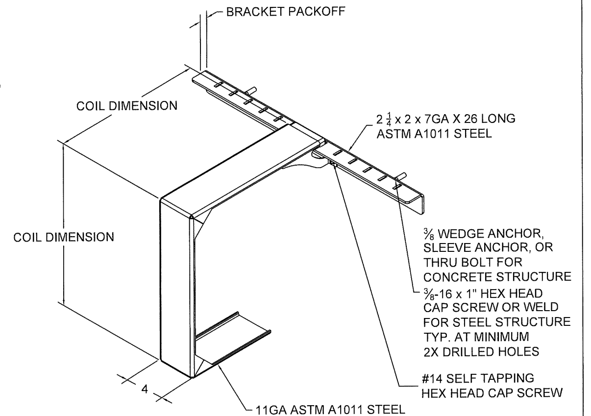
15 MID-HOOD SUPPORT (WHEN REQUIRED)
