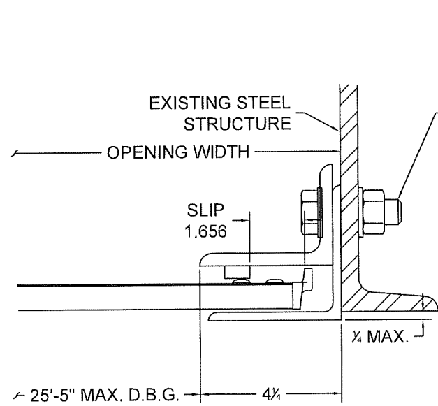
12 GUIDE ASSEMBLY STEEL STRUCTURE (BETWEEN JAMBS GUIDE)
