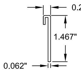
⑱* SILL RISER, FLAT, 1-1/2"*
