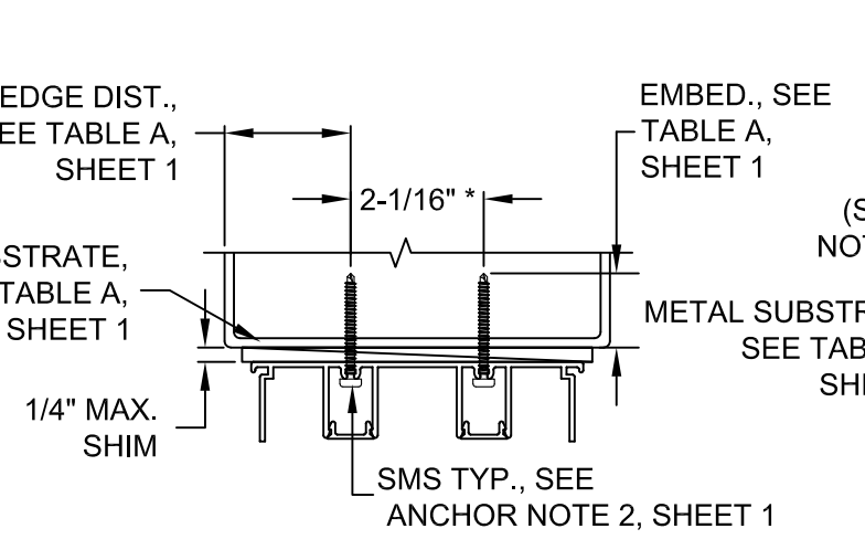
DETAIL E 2-TRACK FRAME HEAD WOOD INSTALLATION
