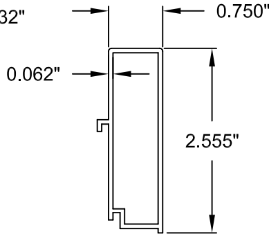
㉑ SILL RISER, BOX, 2-1/2"
