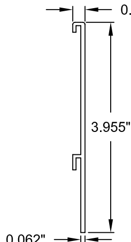
㉔ SILL RISER, FLAT, 4"
