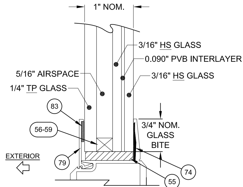
1" LAMINATED INSULATING GLASS TYPE G9A
