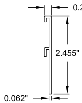
⑳ SILL RISER, FLAT, 2-1/2"
