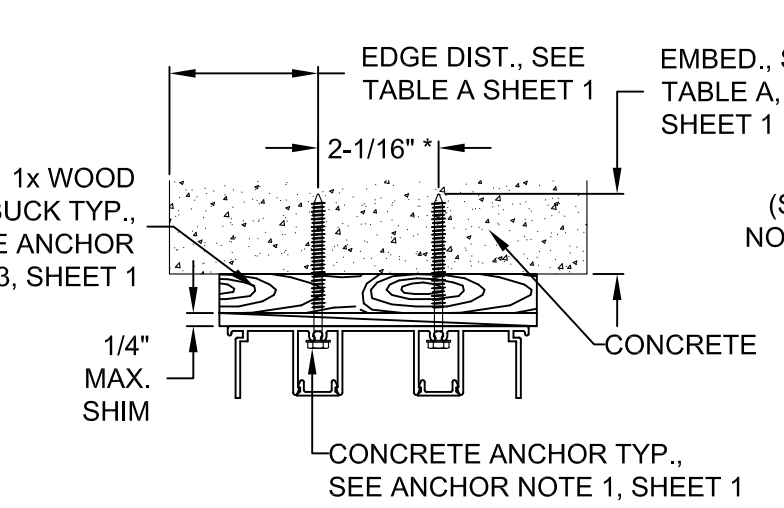
DETAIL E 2-TRACK FRAME HEAD CONCRETE INSTALLATION
