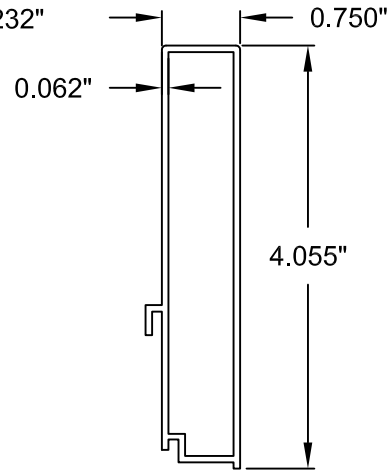
㉕ SILL RISER, BOX, 4"
