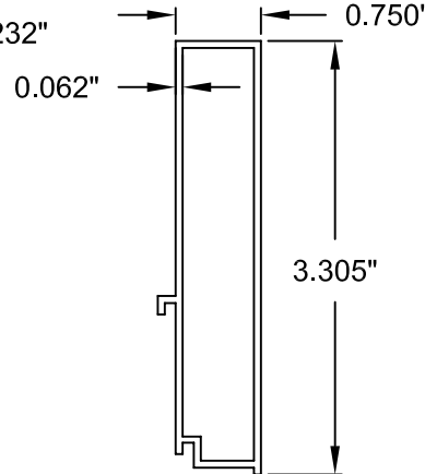
㉓ SILL RISER, BOX, 3-1/4"
