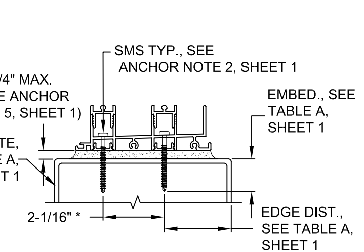
DETAIL F 2-TRACK FRAME SILL WOOD INSTALLATION
