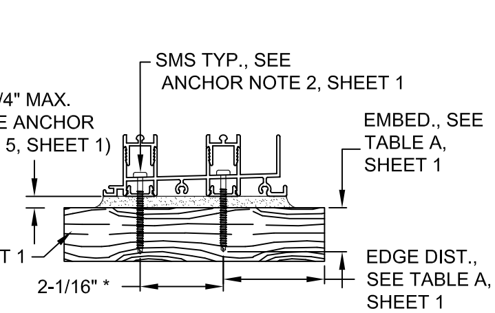
DETAIL F 2-TRACK FRAME SILL WOOD INSTALLATION
