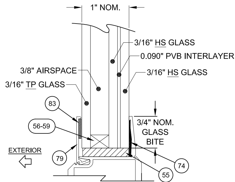
1" LAMINATED INSULATING GLASS TYPE G9
