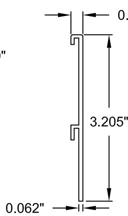
㉒ SILL RISER, FLAT, 3-1/4"
