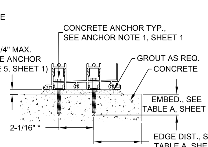
DETAIL F 2-TRACK FRAME SILL CONCRETE INSTALLATION
