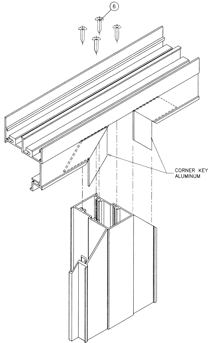
IMPOST CORNER
