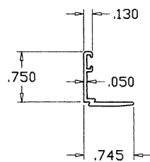
GLAZING BEAD
