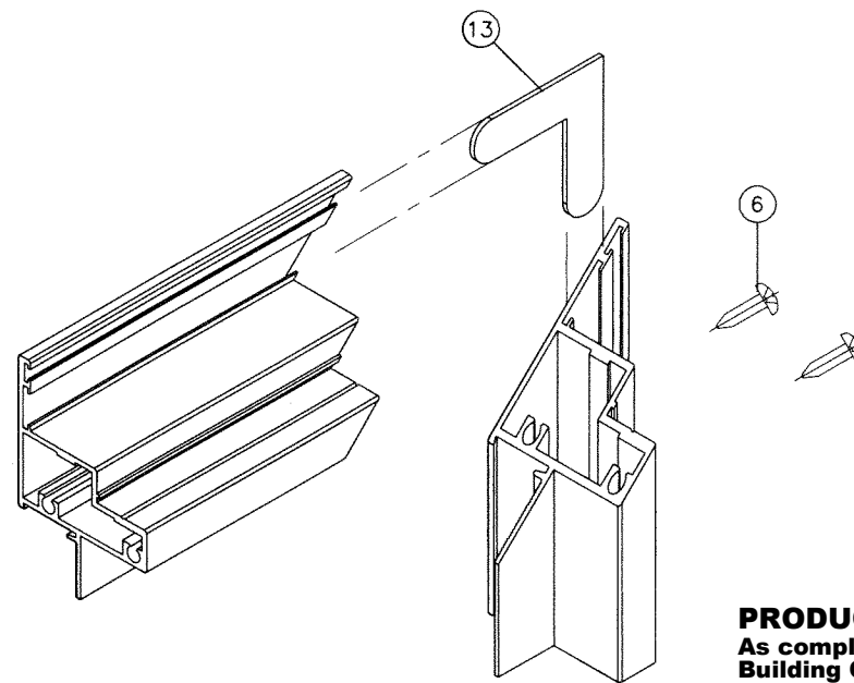
VENT CORNER
