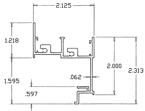
FRAME
