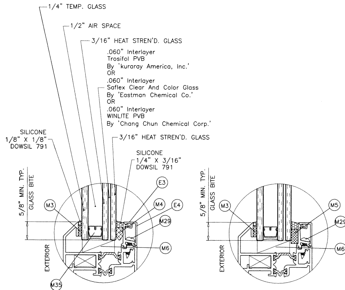
GLASS TYPE 'B' 1-3/16" OVERALL NOM. THK.
